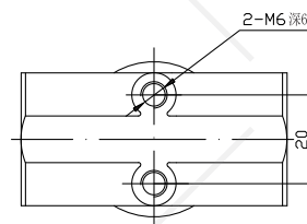
G3/8"-G1/2" 阀体底部安装孔
