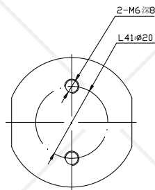
G1/4" 阀体底部安装孔
