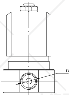
G1/4" 阀体底部安装孔
